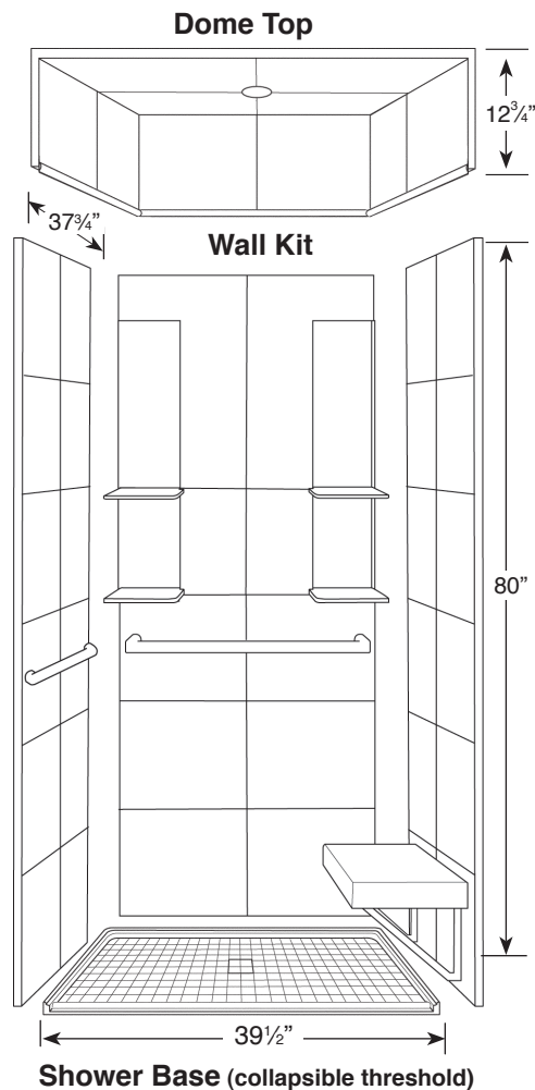
Shown with FC3938 Shower Base, T3981 Dome Top and GB1529PS Grab Bar set, GBHS18PS Hand Shower
